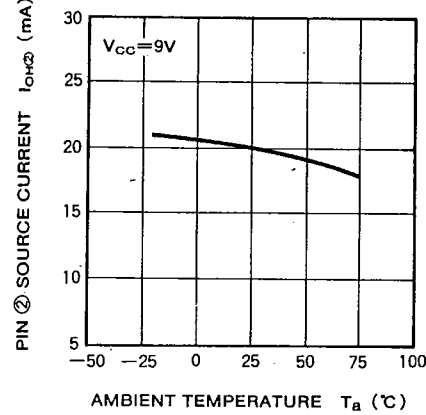
PIN ② SOURCE CURRENT VS. AMBIENT TEMPERATURE
